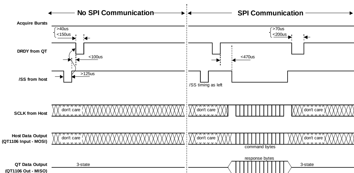
Figure 4.2 LP Mode SPI Operation with LPB = 0
