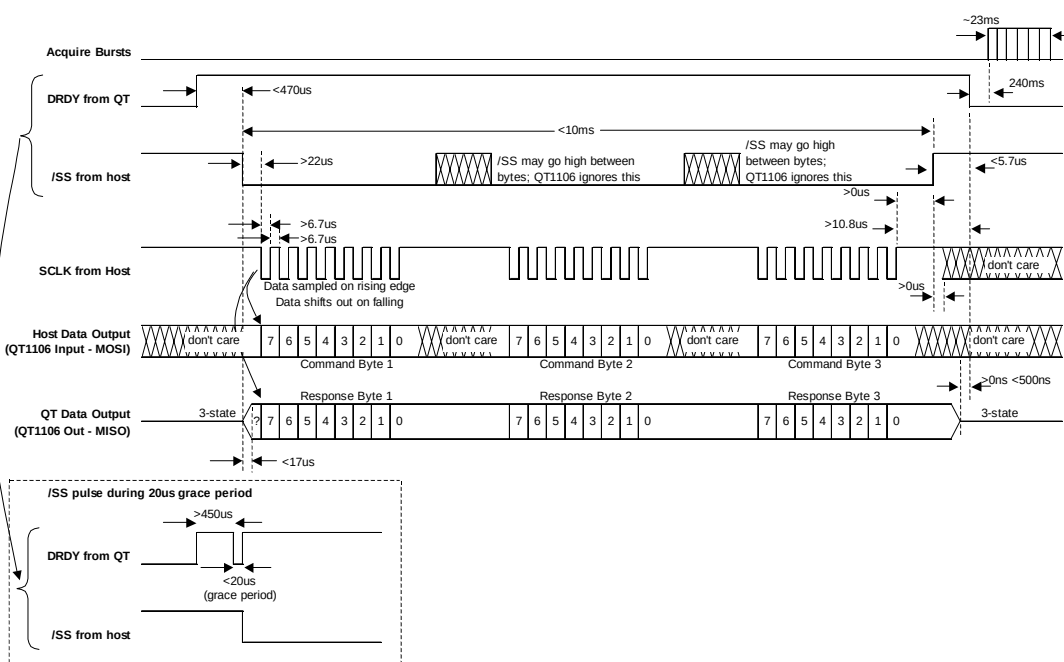
Figure 3.1 SPI Operation
